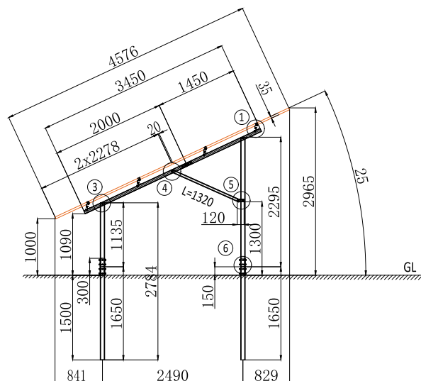
FS-Support 25°-2P Side View Scale 1:1
